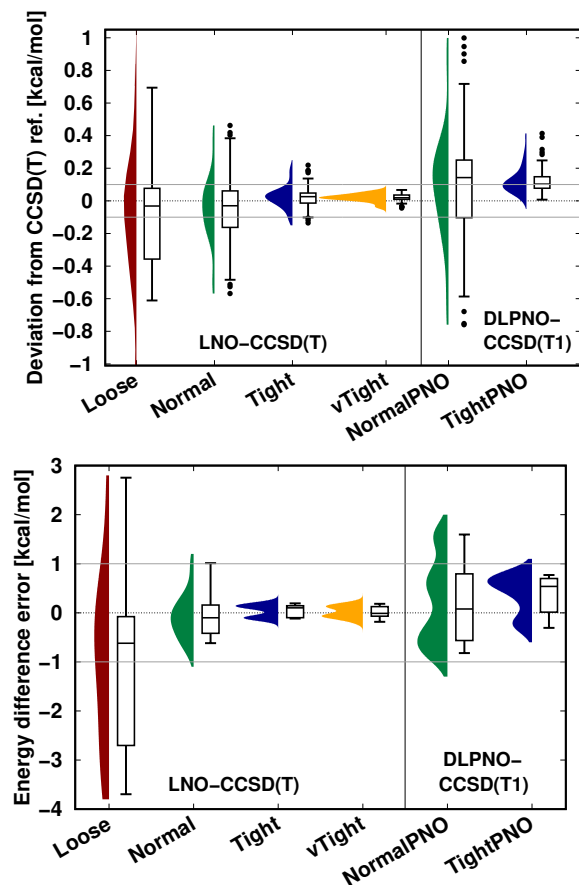
Fig. 9 LNO-CCSD(T) (left) and DLPNO-CCSD(T 1 ) (right) energy deviations against the DF-CCSD(T) reference for the S66 153 interaction energy compilation in the haug-cc-pVTZ basis set 149 (top panel) and the CEMS26 compilation 29 (bottom panel). (Half) violin curves show the distribution of the signed errors, where the height of the curve (along the horizontal axis) indicates the frequency of the signed errors corresponding to an error value on the vertical axis. The horizontal lines of the boxes indicate the lower, median, and upper quartiles, respectively. Whiskers extend to the most distant data point whose error value lies within 1.5 times of the difference between the lower and upper quartiles. Outliers beyond the whiskers, if any, are represented by dots. The numerical data is from Tables 3 and S2 of Ref. 29.
