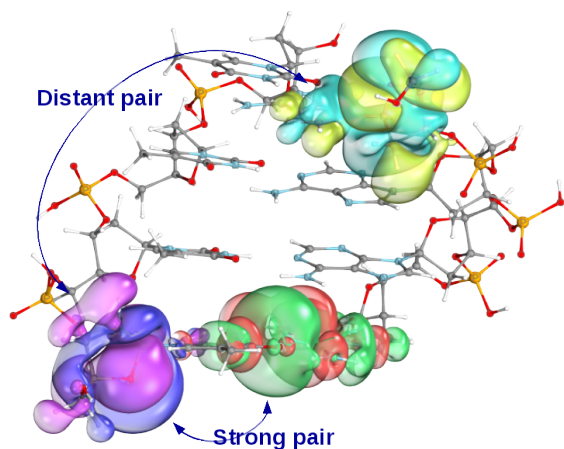
Fig. 2 Strong (red-green) and distant (yellow-cyan) local MO pair of a selected local MO (purple-pink) for a four base-pair DNA fragment. The LMO isosurfaces are selected to encompass 99.99% of the LMO.
