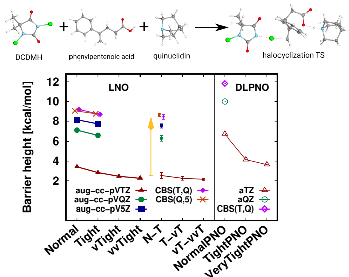
Fig. 6 Transition state (63 atoms) barrier height of a halocyclization reaction comparing LNO-CCSD(T) (left) and DLPNO-CCSD(T 1 ) (right) barrier height energies. 150,154 The CBS(T,Q) and CBS(Q,5) LNO-CCSD(T) results are slightly shifted along the x-axis to increase visibility.
