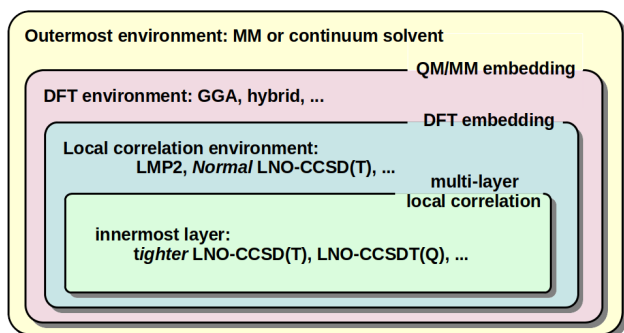
Fig. 3 Illustration of the QM/MM, DFT, and multi-layer local correlation embedding variations available in the MRCC 58,59 package.
